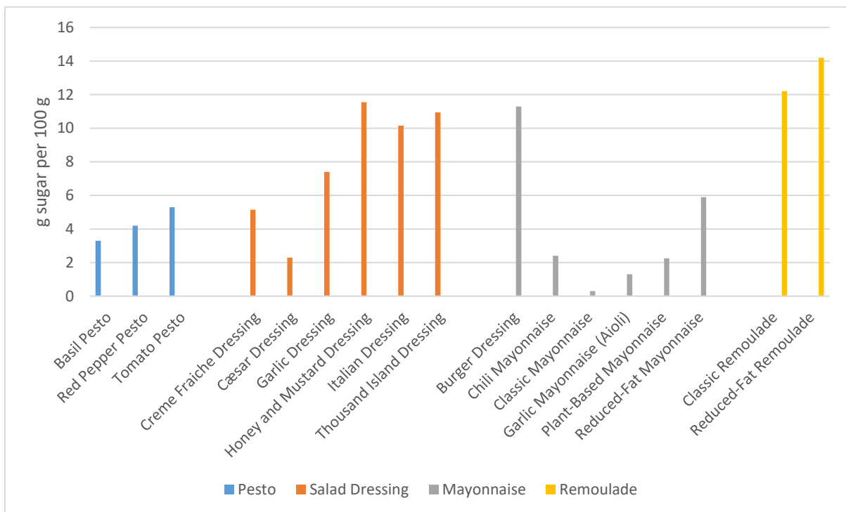
Figure 5. Sugar content (g per 100 g) in all composite samples, calculated as the sum of mono- and disaccharides (Appendix C). Values below the limit of quantification were assigned a value of zero.
