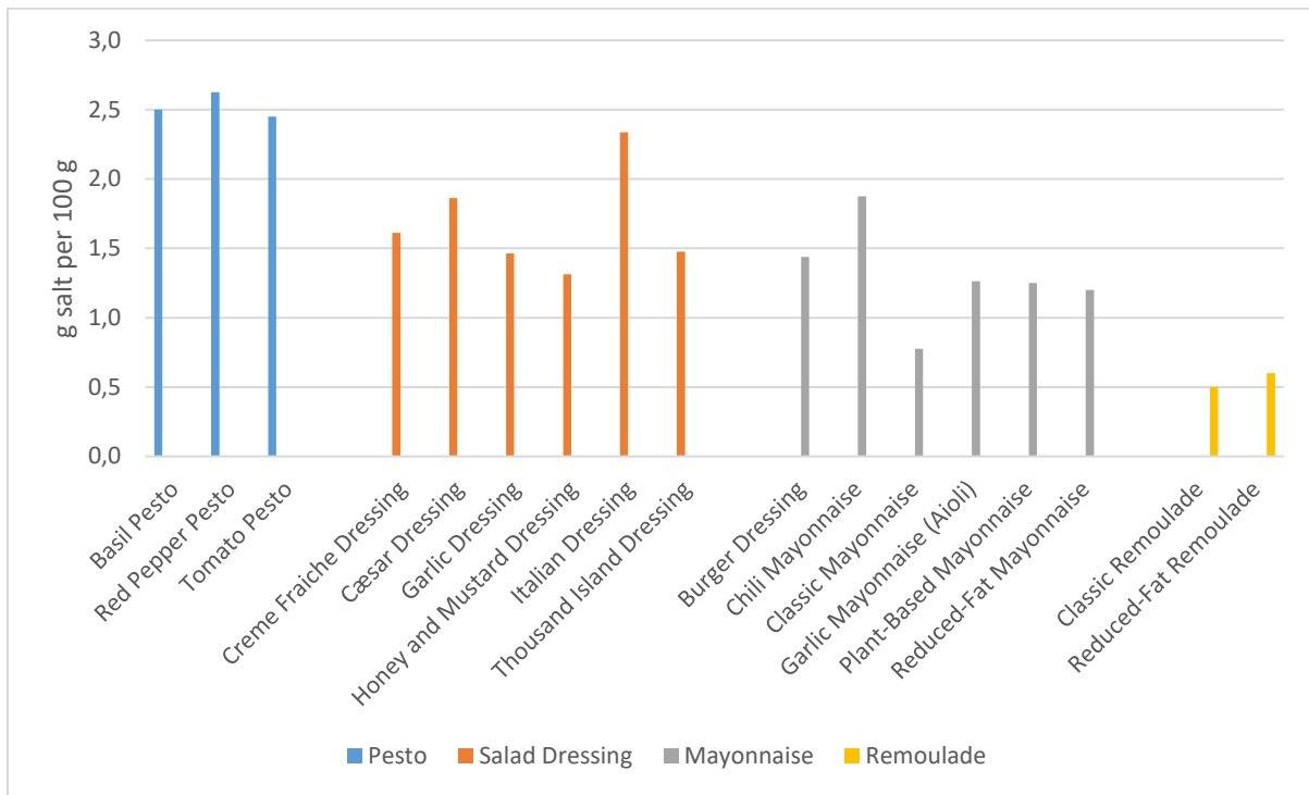
Figure 4. Salt content (g per 100 g) in all composite samples, calculated as 2.5 times the sodium content (Appendix E).
