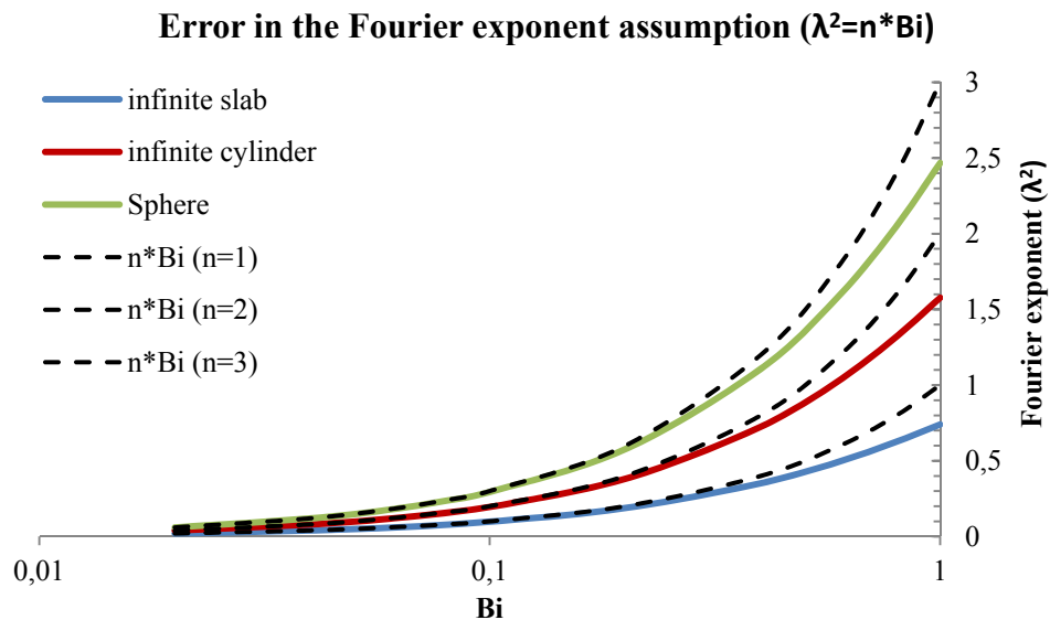
Figure 7.2 The error induced in the Fourier exponent determination by the lumped capacity assumption for the 3 elementary geometries
