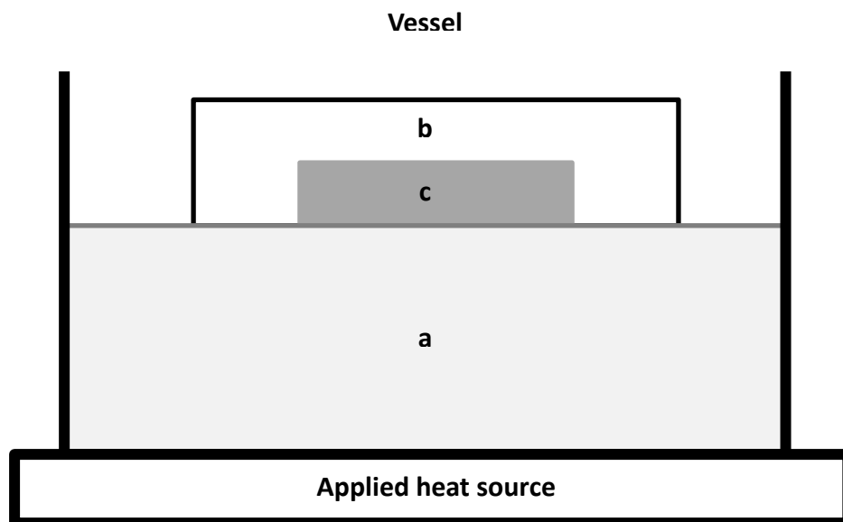
Figure 1 Schematic experimental setup for determination of heat transfer coefficients. Domain a is the heating media, for this experiment three different types of soups, and water was used. Domain b is a polystyrene mold used to insulate the aluminum block. Domain c is the aluminum block.
